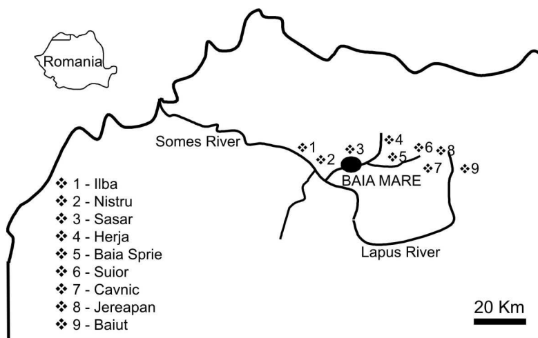
Fig. 1. Location of Băiut area in Baia Mare metallogenetic district. Legend: 1 to 9 – metallogenetic fields
