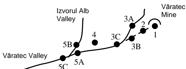
Fig. 5. Sketch with the samples location from the Văratec Băiuț area (no scale)
