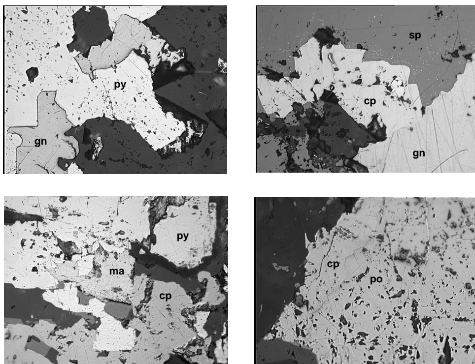
Fig. 3. Microscopic photographs (reflected light, plane polars) of the main sulfides from Văratec Băiuț ore. Legend: py – pyrite, cp – chalcopyrite, gn – galena, sp – sphalerite, ma – marcasite, po – pyrrhotite
