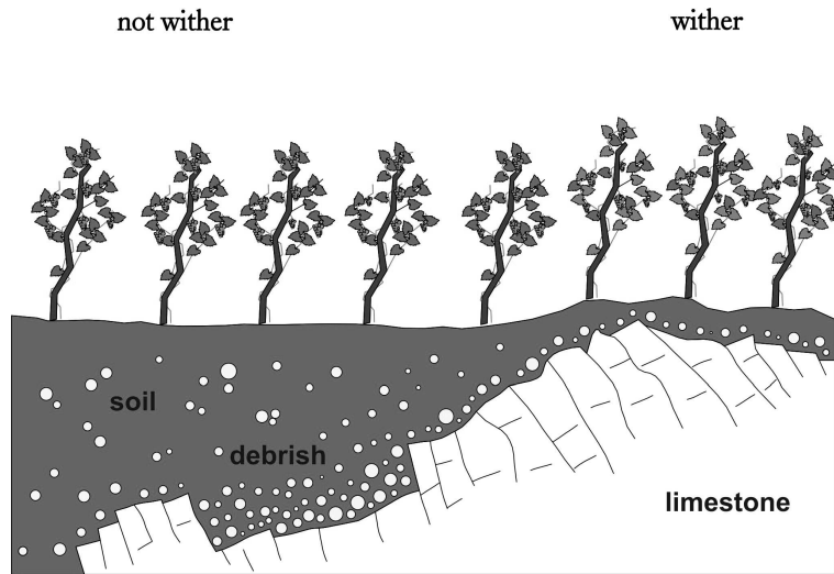
Fig. 3. Chlorosis type 1 (Limestone basic rocks)
