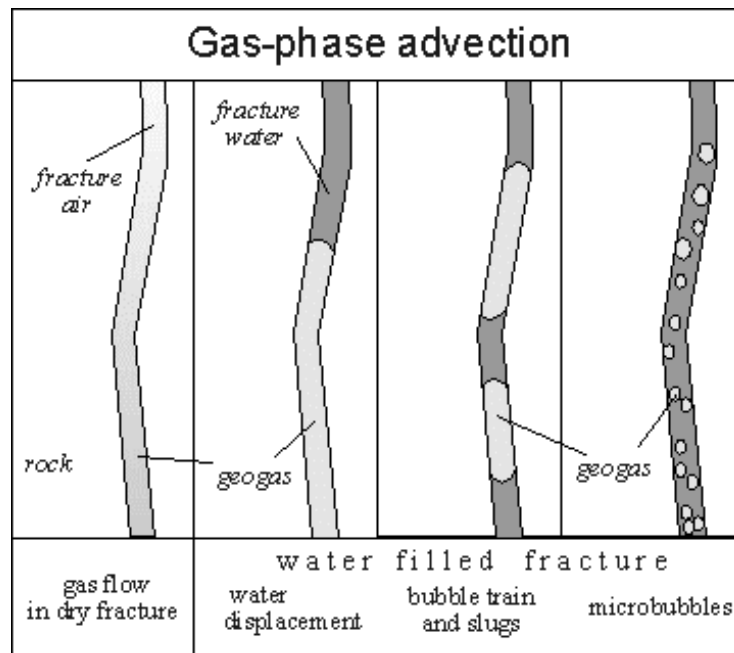
Fig. 2. Schematic picture of gas-phase advection forms. For all forms the flow is controlled by permeability (fracture aperture for bubble flows) and pressure gradients, that may be induced by tectonic stresses, fracturing, variations of lithostatic loading, aquifer or fluid reservoir charge/discharge, local gas production, and barometric pumping near the surface (from Etiope and Martinelli, 2002)
