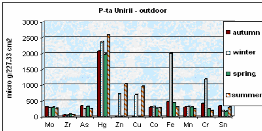
Fig. 3. Heavy metals concentration in P-ta Unirii (outdoor)
