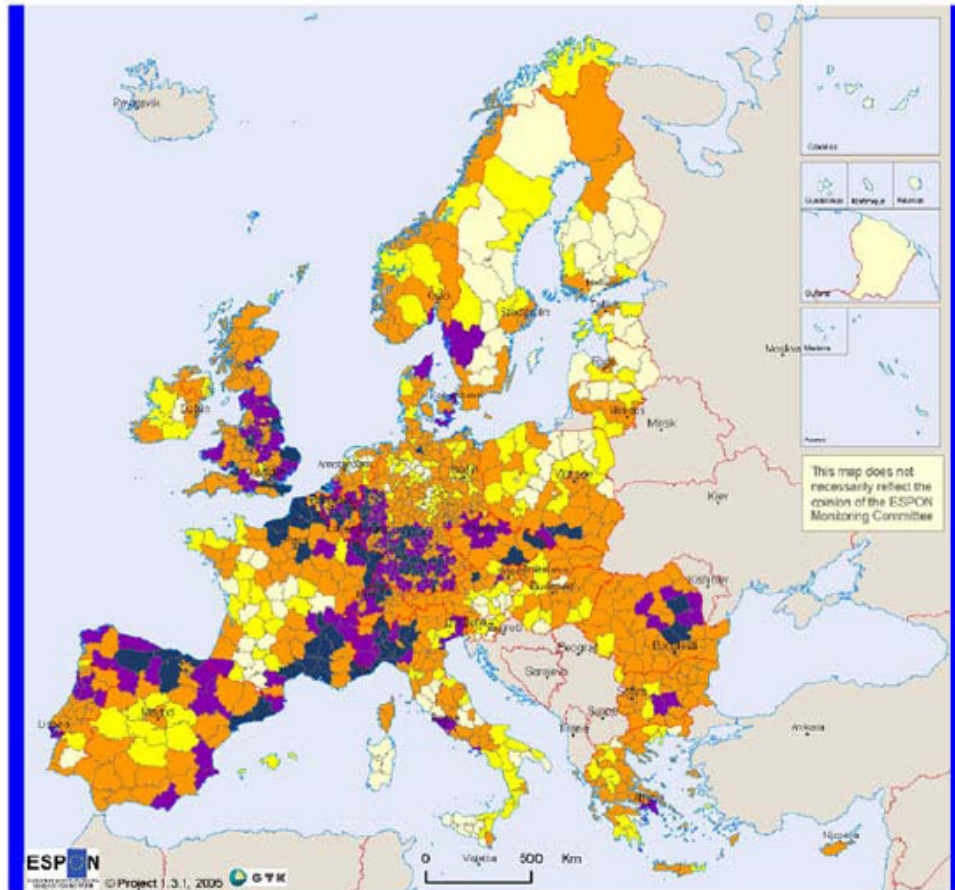
Plate II . Probability occurrence map of the landslides at the administrative level in EU
