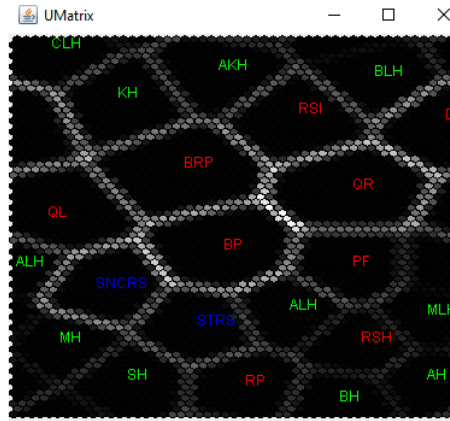
FIGURE 6. U-Matrix visualization.
